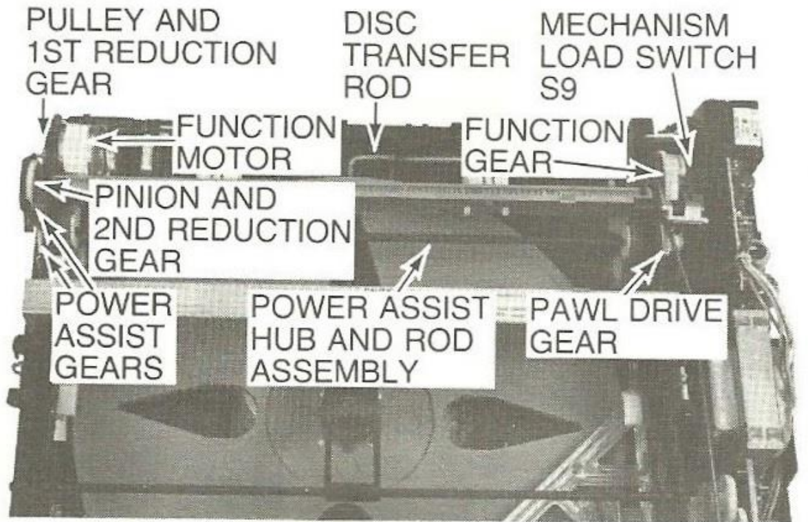
Fig. 4—Mechanism Identification
